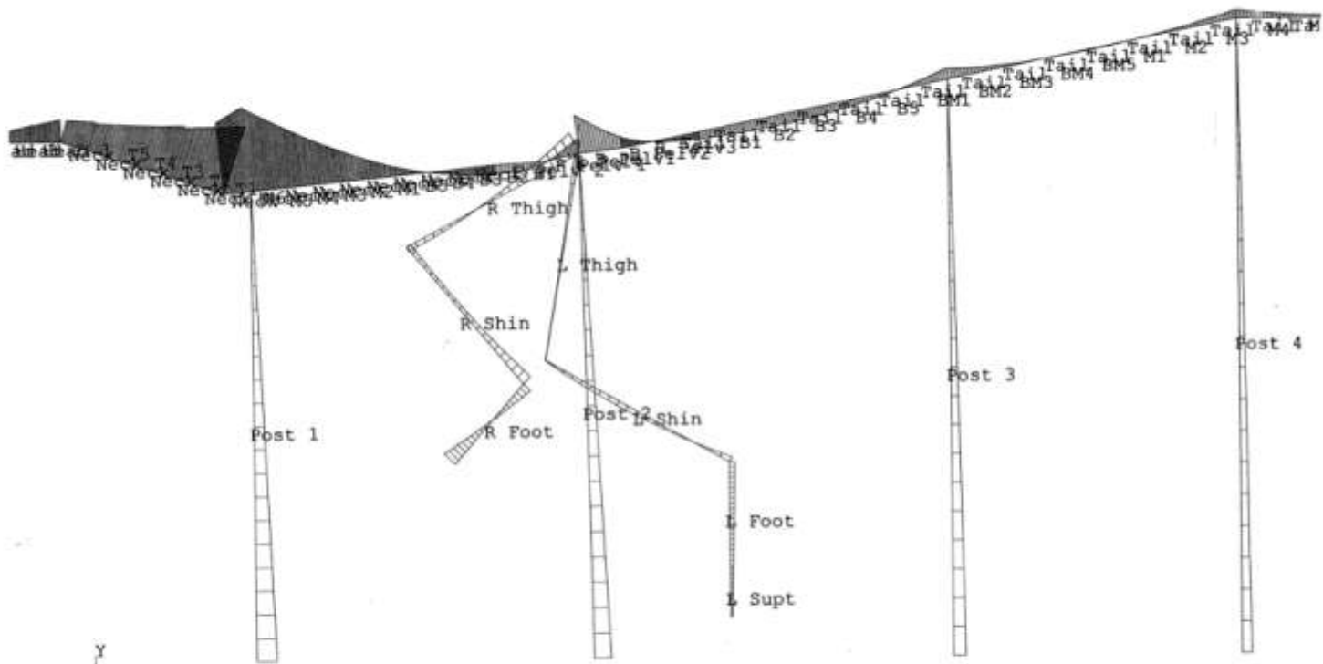
BENDING MOMENTS FIG. 7
