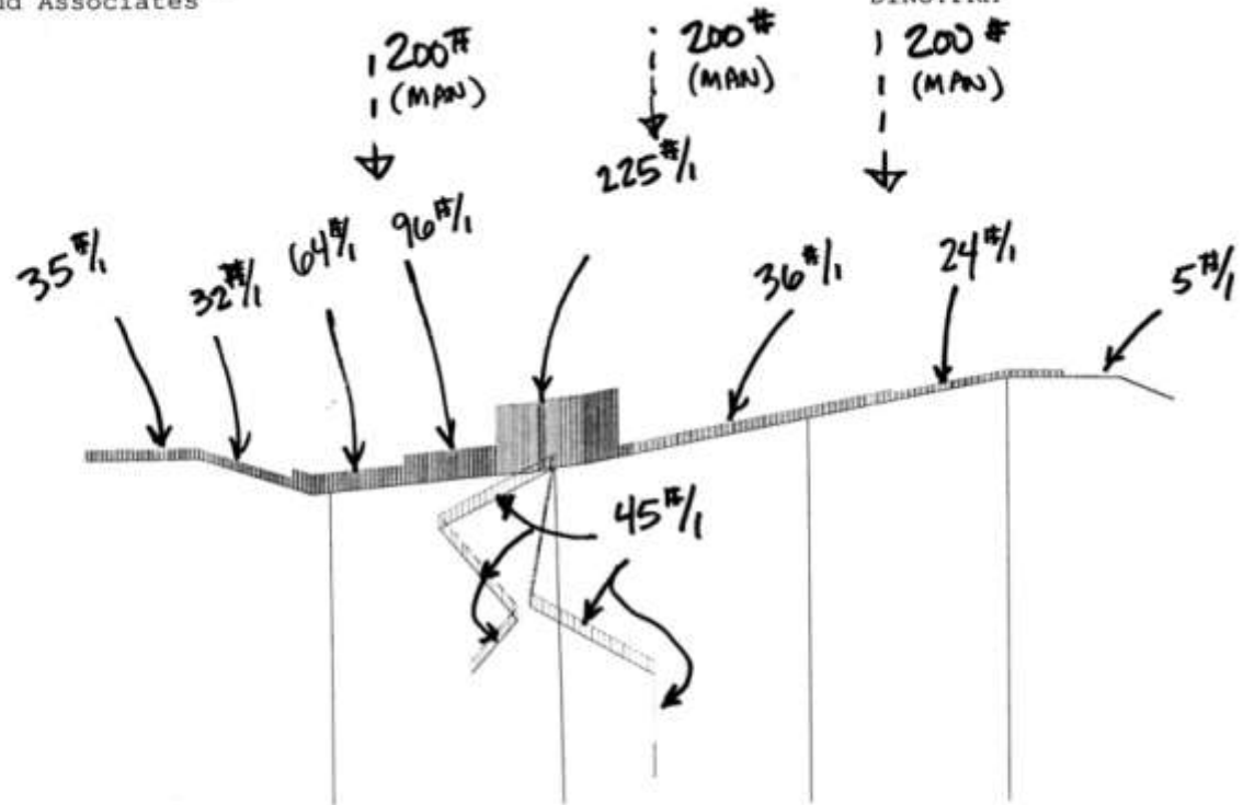
LOADS P 0 MODEL FIG. #5
